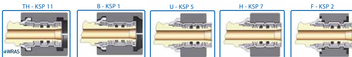
Profile and dimensions of the jaws that can be used with Multi-Jaw Gerpex Fittings
